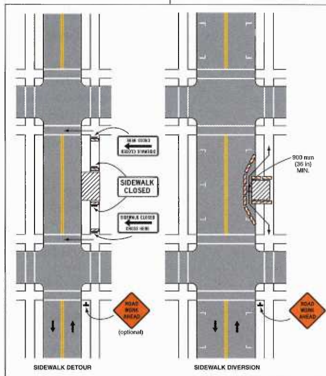
Exhibit 4-14. Accommodating Pedestrians at Midblock Construction Zones (6).
