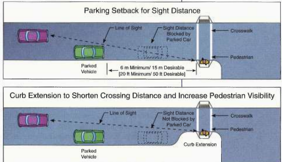
Exhibit 3-3. Recommended Parking Setback and/or Curb Extension Installation (18).
