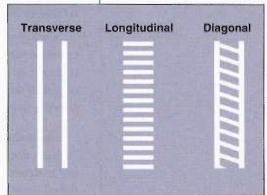
Exhibit 3-25. Crosswalk Marking Options.
