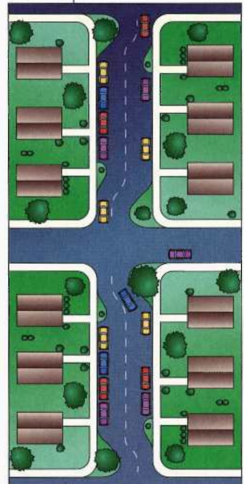
Exhibit 2-13. Chicanes.
