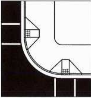
Exhibit 3-30. Perpendicular Ramps (13).
