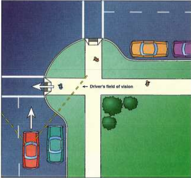
Exhibit 3-22. Example of Curb Extension Design (13).
