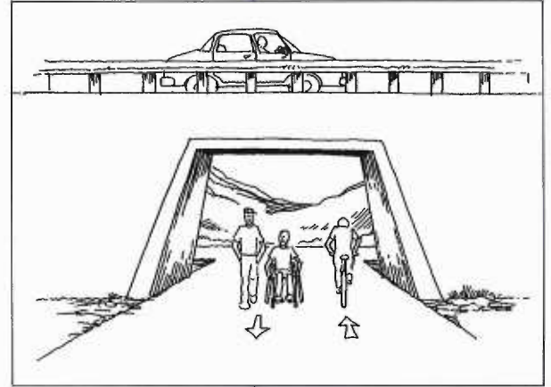
Exhibit 3-40. Convenient and Open Underpass Design (20).
