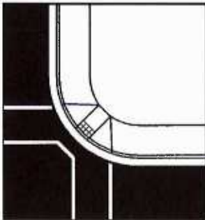
Exhibit 3-32. Diagonal Ramp (13).
