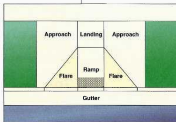
Exhibit 3-26. Standard Curb Ramp Components (13).
