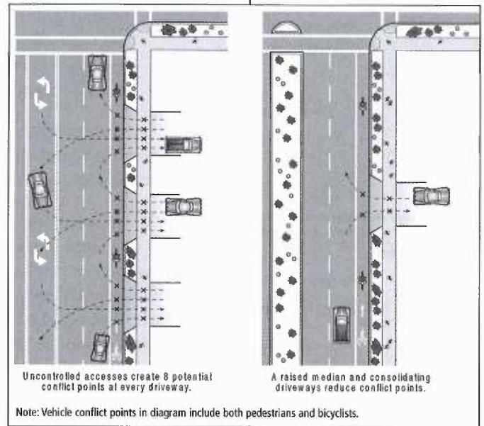
Exhibit 3-8. Uncontrolled Access vs. Controlled Access. (24).
